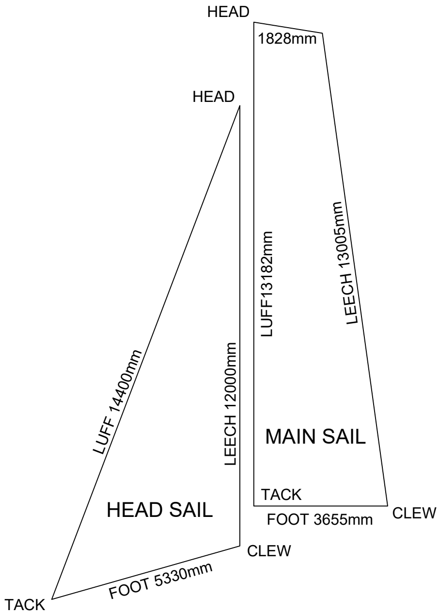
EXISTING SAIL MEASUREMENT
